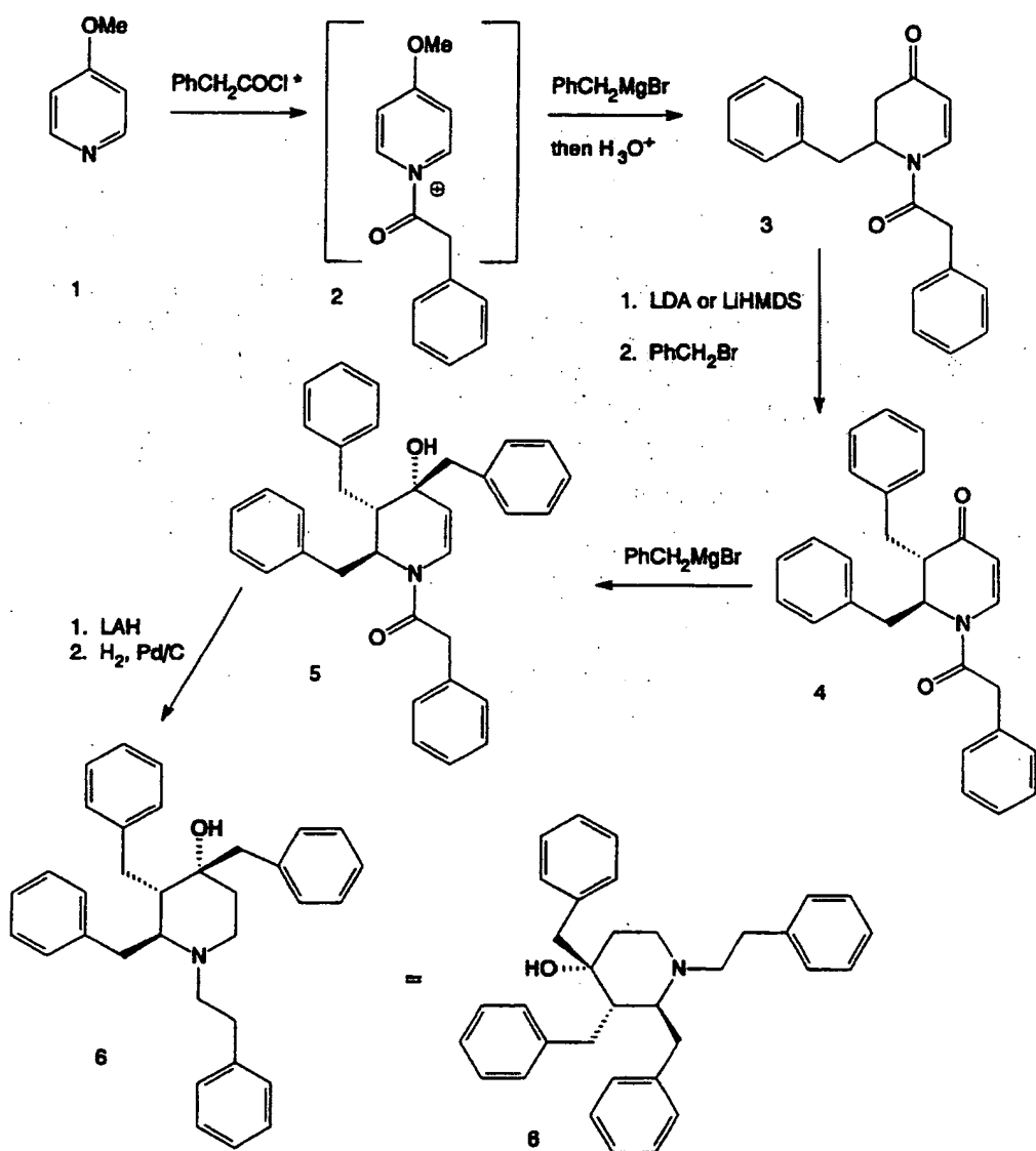
Scheme 3
